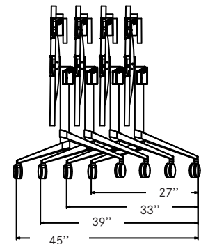
Nesting Configuration: Side view of four tables nested. Approximate dimensions.
