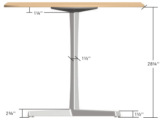
Elevation View of Revue Base
